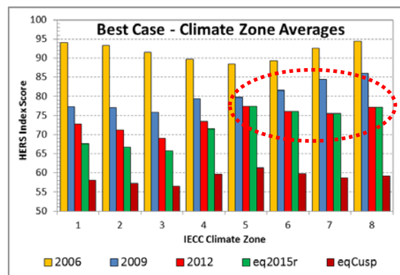
Figure 1b. HERS Index scores for options with vacated gas furnace Rule.
