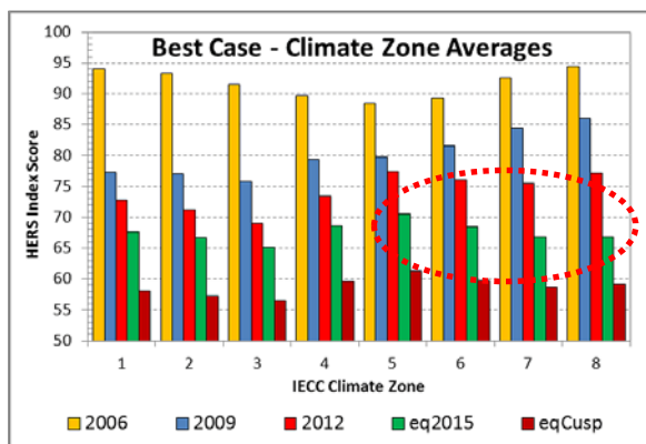
Figure 1a. HERS Index scores for options with original gas furnace Rule.
