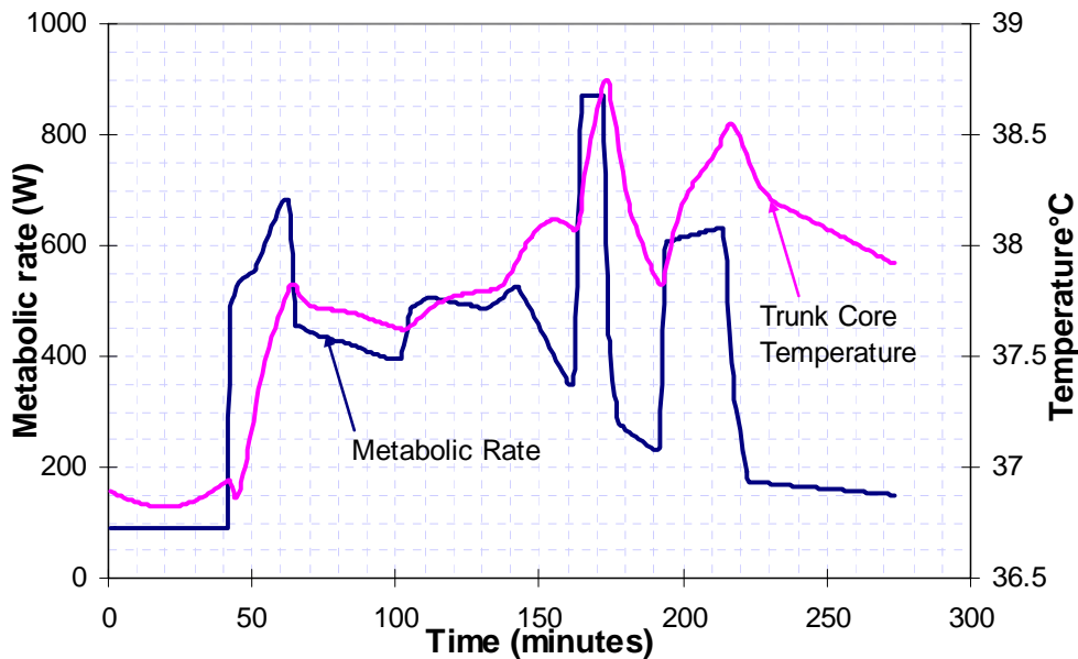
Figure 4.12 Trunk Core Temperature and Metabolic rate
