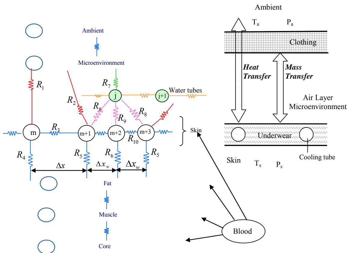
Figure 3.4 Thermal Resistance Network of Thermal Model
