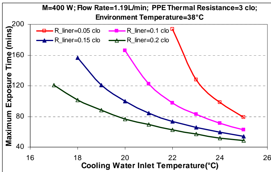
Figure 5.4 Maximum Exposure Time under Various Liner Thermal Resistance and Cooling Water Inlet Temperature
