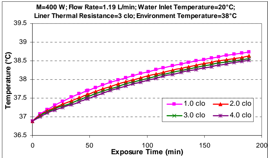
Figure 5.7 Trunk Core Temperature vs. PPE Thermal Resistance
