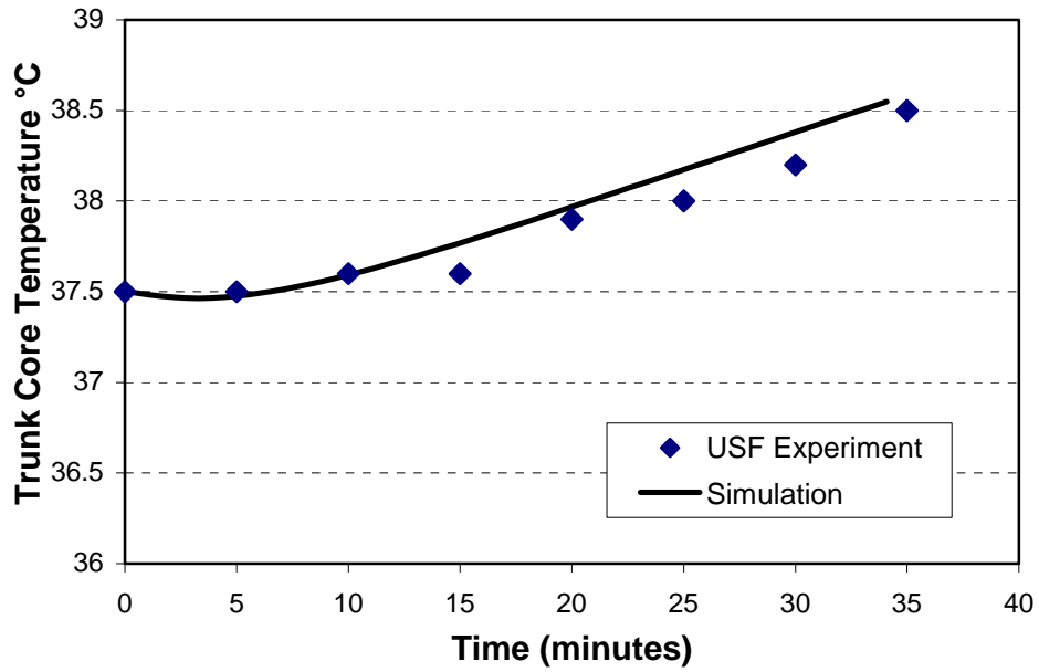
Figure 4.1 Comparison on Control without Cooling between Simulation and USF Experiment—Subject A (M=280 W)
