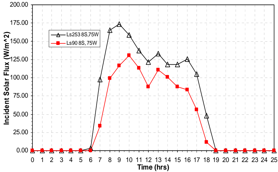
Figure 5.14 Solar insolation Diurnal Mars
