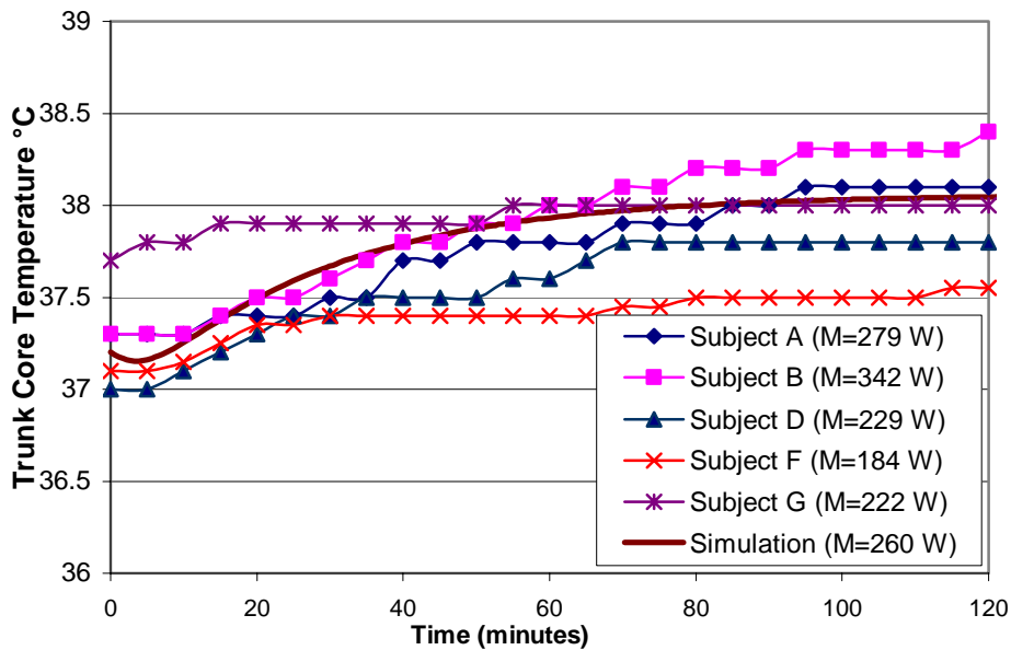
Figure 4.9 Comparison on Air Cooling Vest between Simulation and USF Experiment
