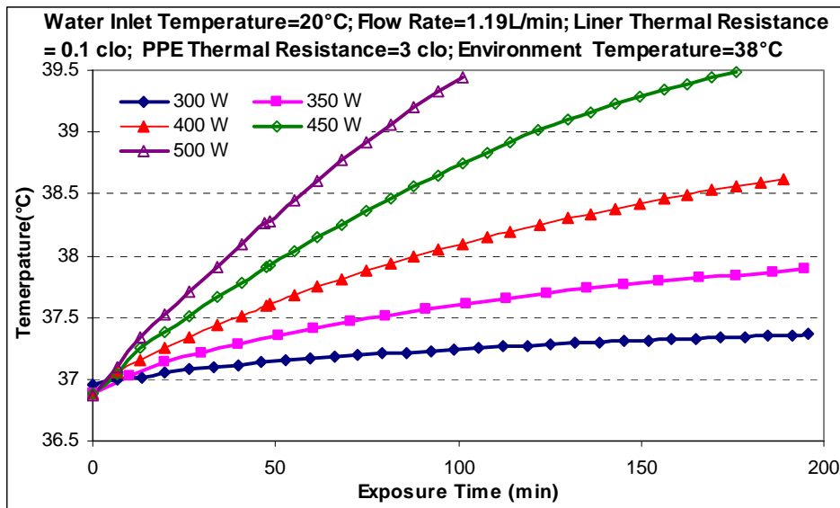
Figure 5.3 Trunk Core Temperature vs. Metabolic Rate with Liquid Cooling Garment
