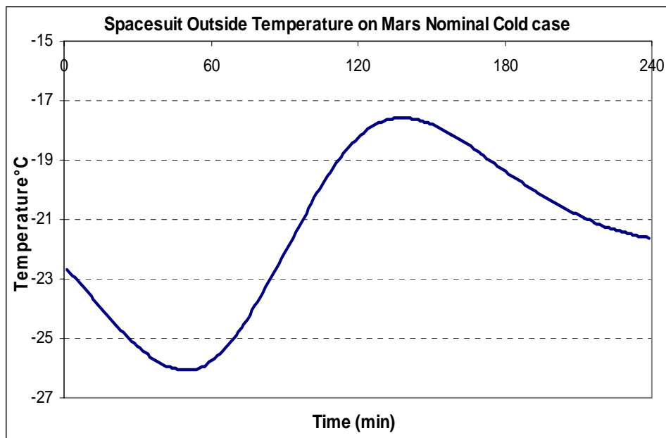
Figure 5.23 Outside Temperature of Spacesuit (Nominal Cold Case)
