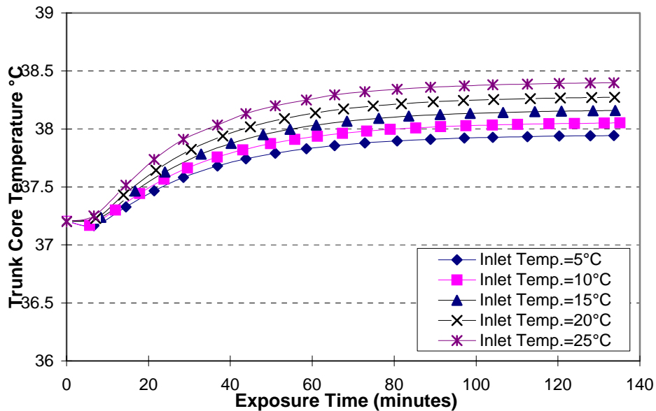
Figure 5.10 Trunk Core Temperature vs. Inlet Cooling Air Temperature (M=260W, Cooling Air Flow Rate=10 CFM)
