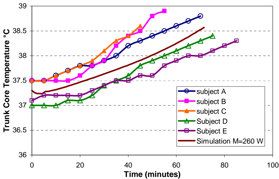
Figure 4.10 Comparison on Ice Cooling Vest between Simulation and USF Experiment
