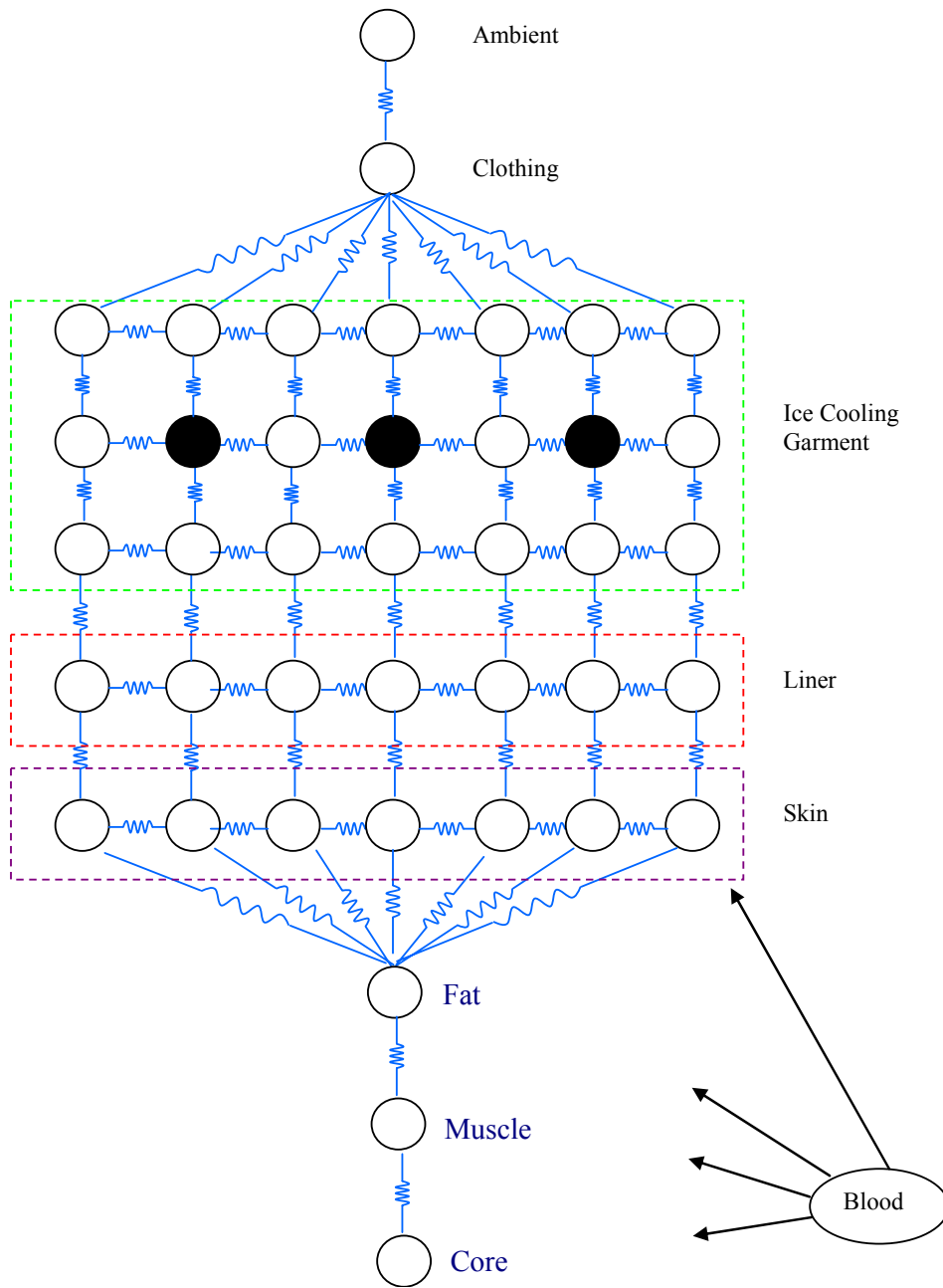
Figure 3.9. Ice Cooling Model Nodes Network
