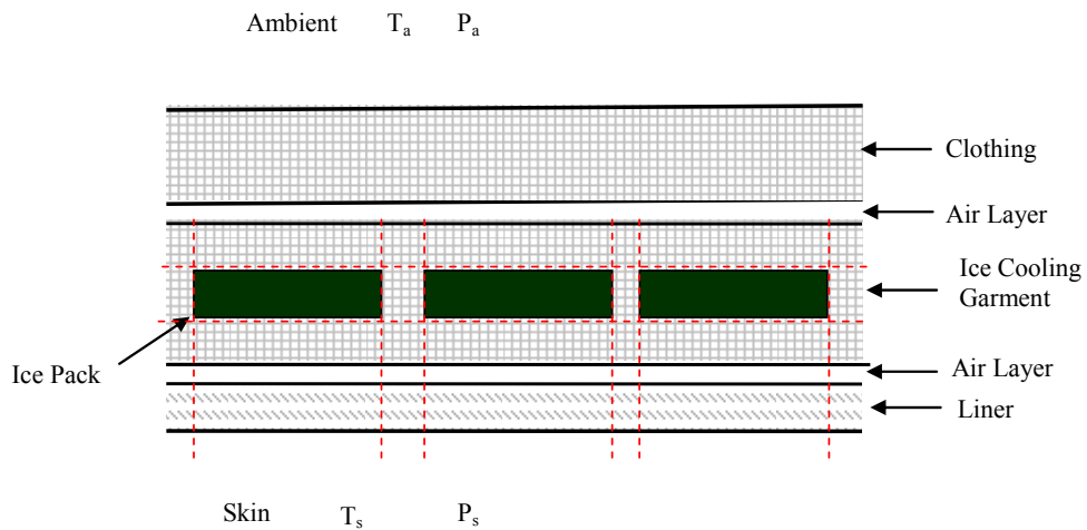
Figure 3.8. Ice Personal Cooling Vest
