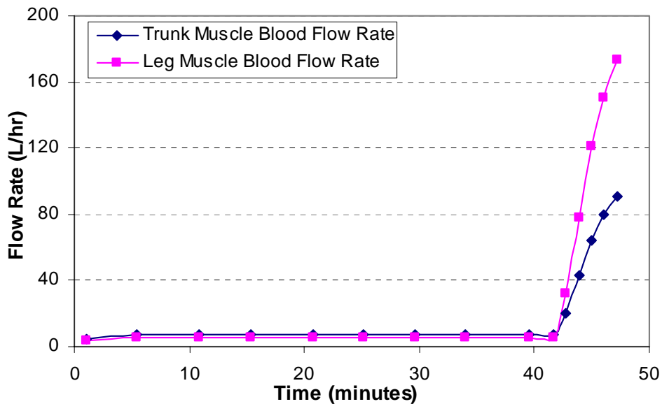
Figure 4.15 Trunk and Leg Muscle Blood Flow Rate
