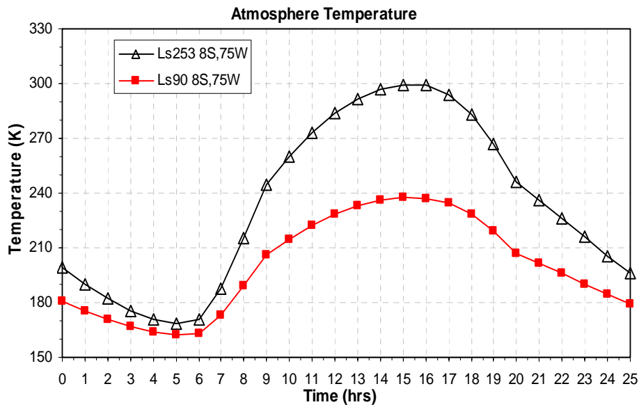
Figure 5.15 Temperature on Mars Atmosphere
