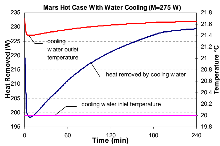
Figure 5.20 Heat Removing , Inlet and Outlet Cooling Water Temperature
