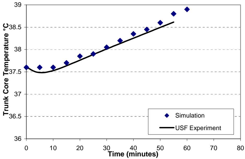
Figure 4.3 Comparison on Water Cooling Vest between Simulation and USF Experiment—Subject A (M=318 W)
