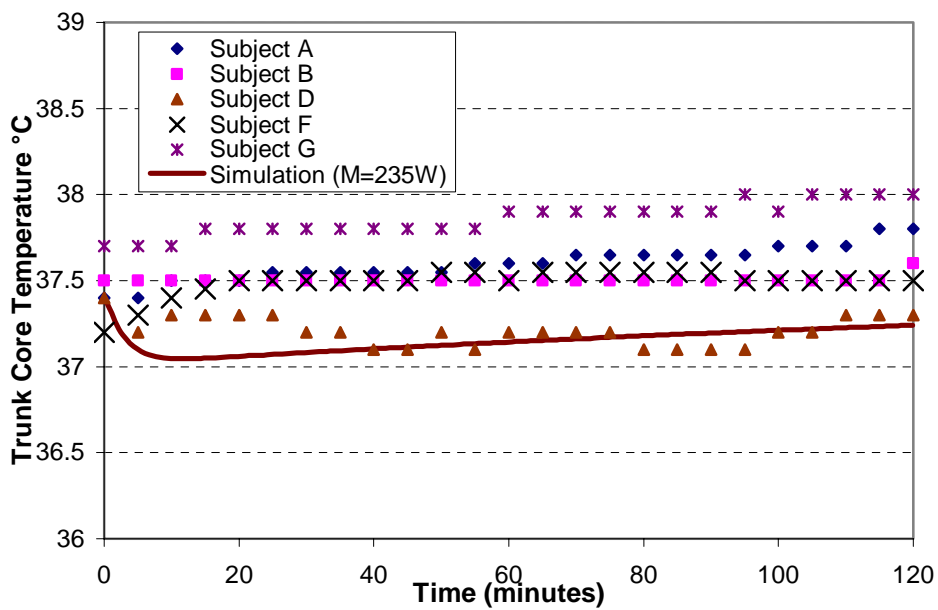
Figure 4.8 Comparison on Water Cooling Suit between Simulation and USF Experiment
