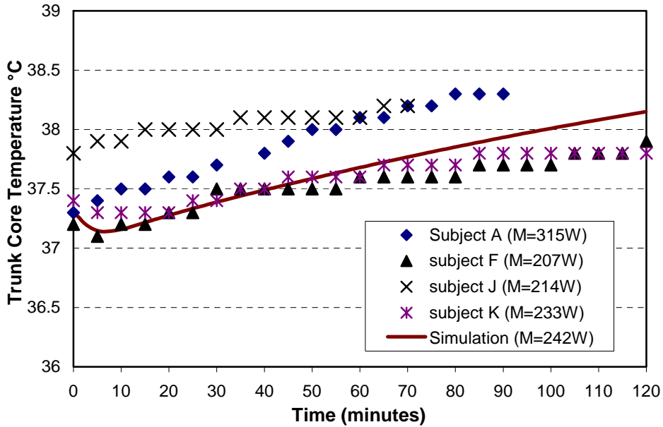
Figure 4.6 Comparison on Water Cooling Jacket between Simulation and USF Experiment
