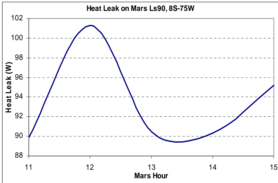
Figure 5.22 Heat Leak from Human Body to Environment (Nominal Cold)
