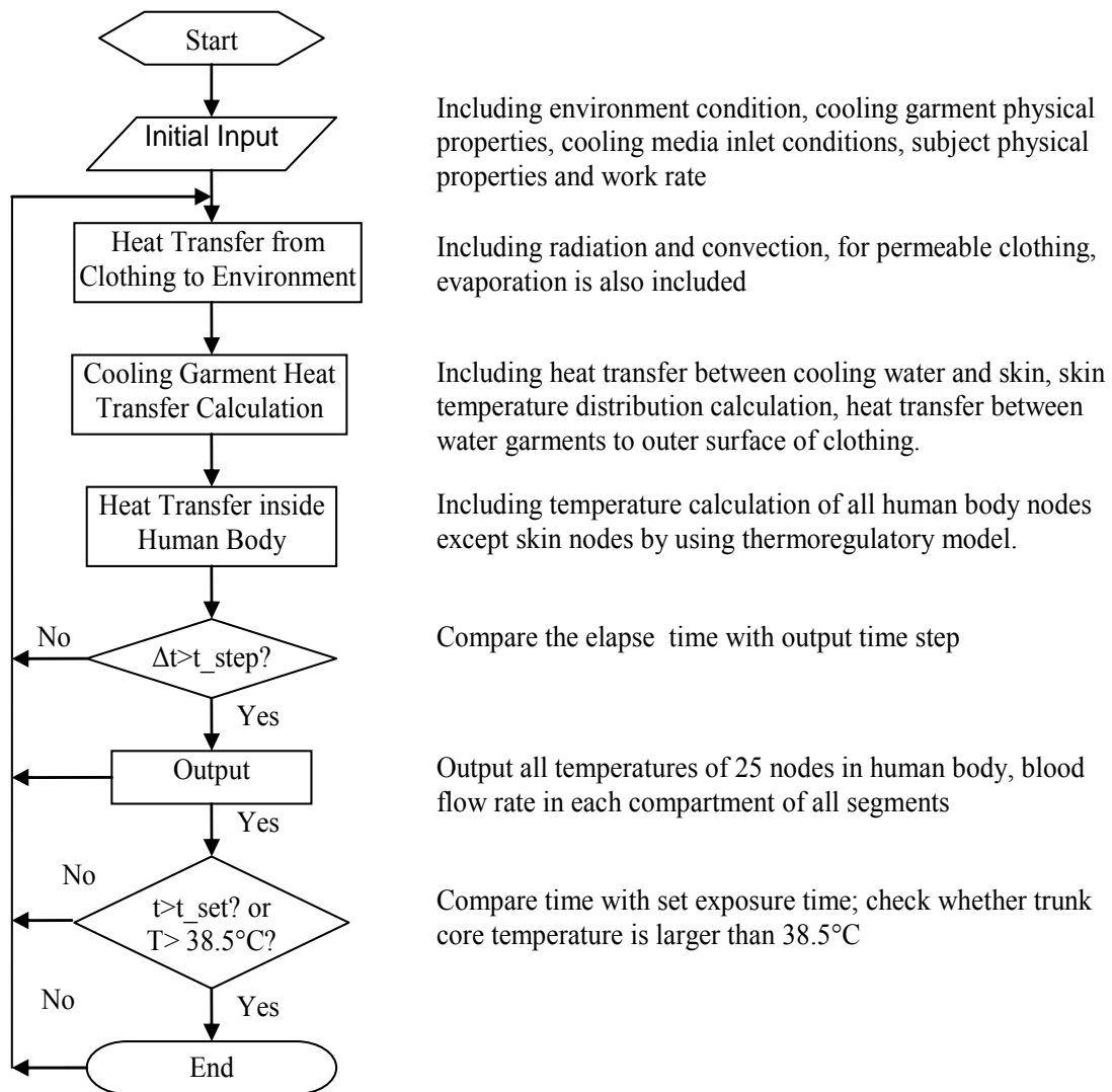
Figure 3.10 Flow Chart of Whole Thermal Model
