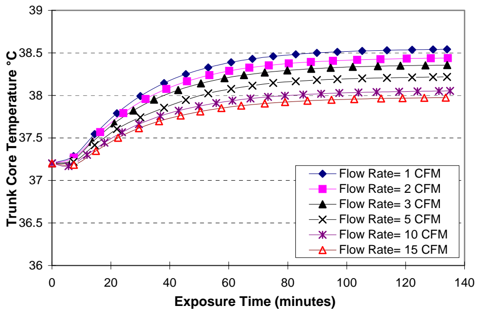
Figure 5.11 Trunk Core Temperature vs. Inlet Cooling Air Flow Rate (M=260W; Cooling Air Inlet Temperature=10°C)
