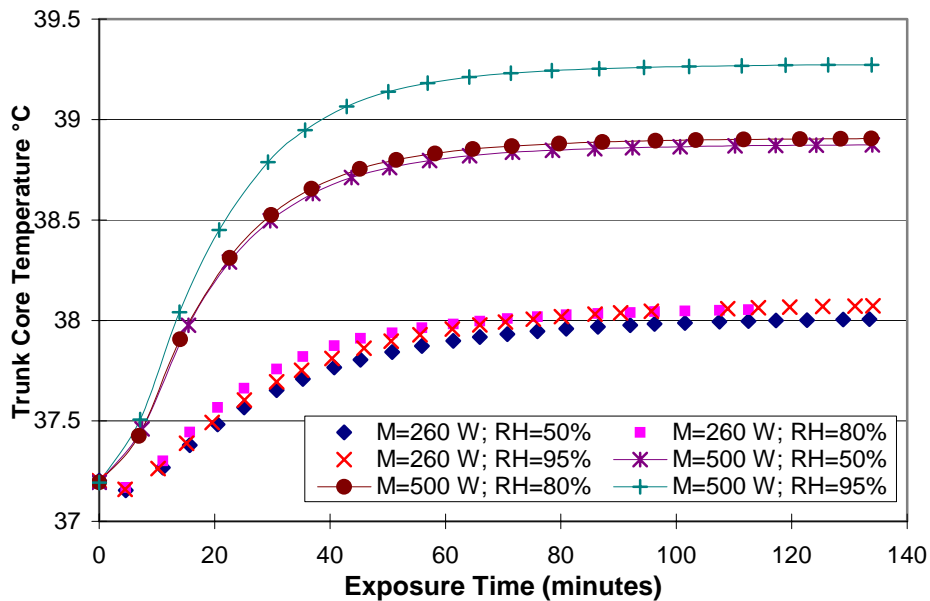
Figure 5.12 Trunk Core Temperature vs. Inlet Cooling Air Relative Humidity (Inlet Cooling Air Temperature = 10°C)
