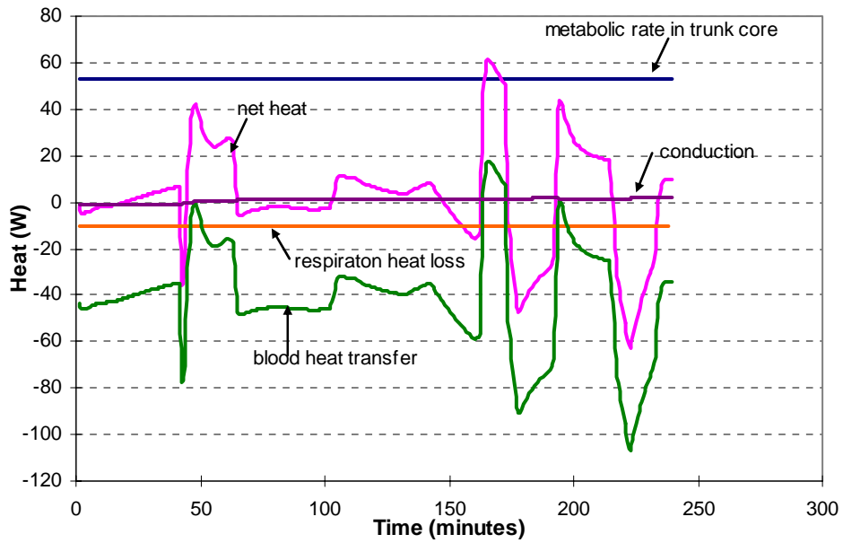
Figure 4.13 Heat Balance in Trunk Core
