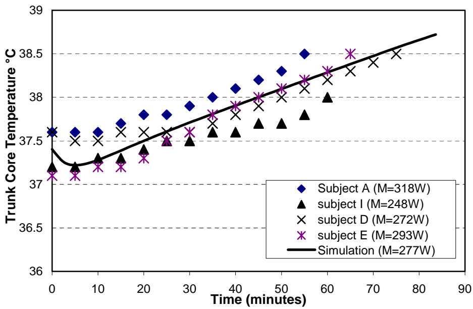
Figure 4.4 Comparison on Liquid Cooling Vest between Simulation and USF Experiment
