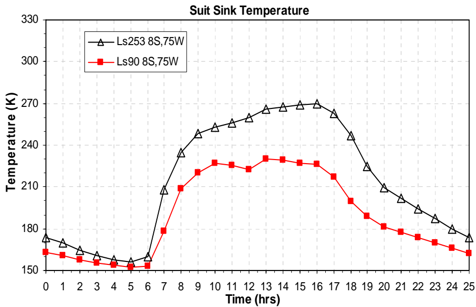
Figure 5.16 Suit Sink Temperature on Mars
