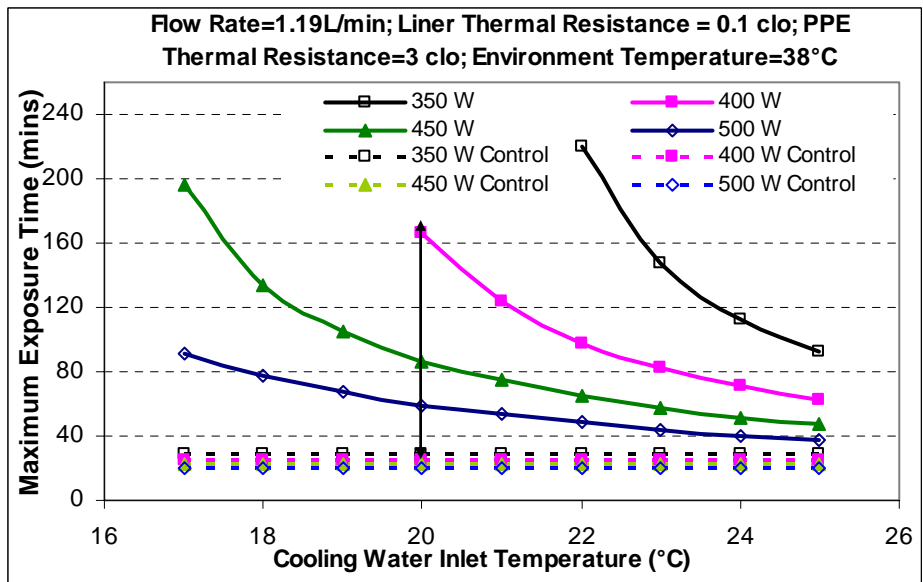
Figure 5.8 Maximum Exposure Time under Various Metabolic Rate and Cooling Water Inlet Temperature
