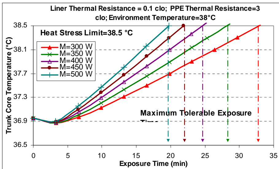
Figure 5.2 Trunk Core Temperature vs. Metabolic Rate without Personal Cooling
