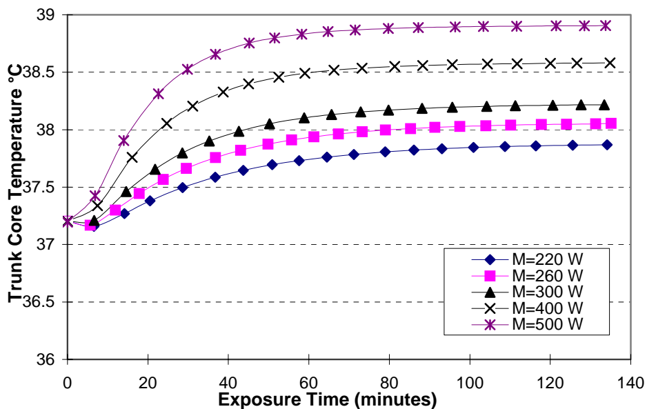
Figure 5.9 Trunk Core Temperature vs. Metabolic Rates (Cooling Air Flow Rate=10 CFM; Inlet Temperature=10°C)
