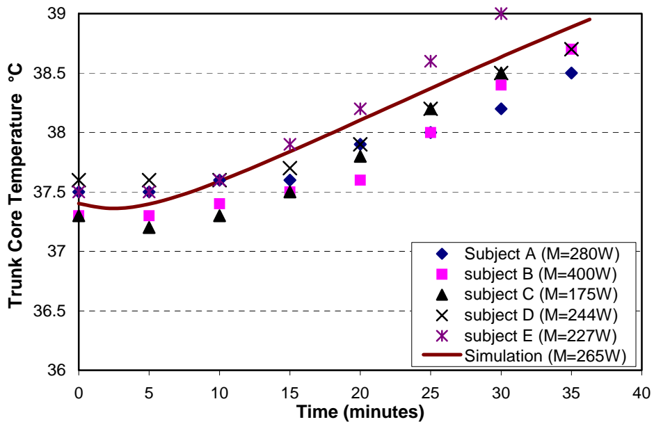
Figure 4.2 Comparison on Control (No cooling) between Simulation and USF Experiment
