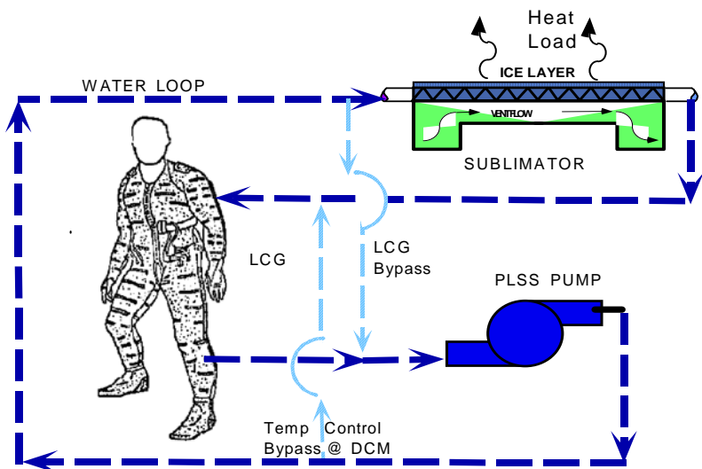
Figure 5.25. Simplified Flow Schematic shuttle EMU Water Loop
