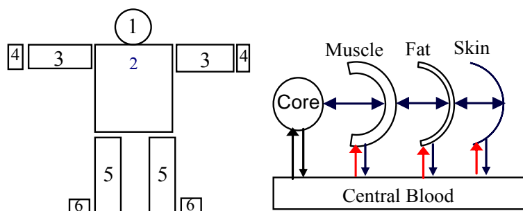
Figure 3.1. Thermoregulatory Model Based on Stolwijk and Hardy
