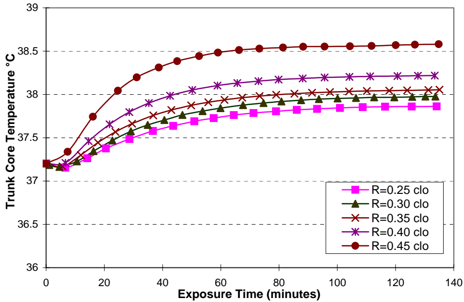
Figure 5.13 Trunk Core Temperature vs. Heat Resistance of T-shirt
