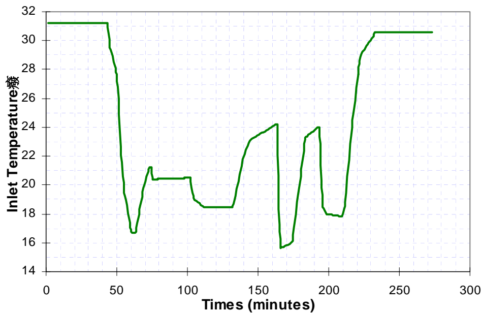
Figure 4.11 Cooling Water Inlet Temperature
