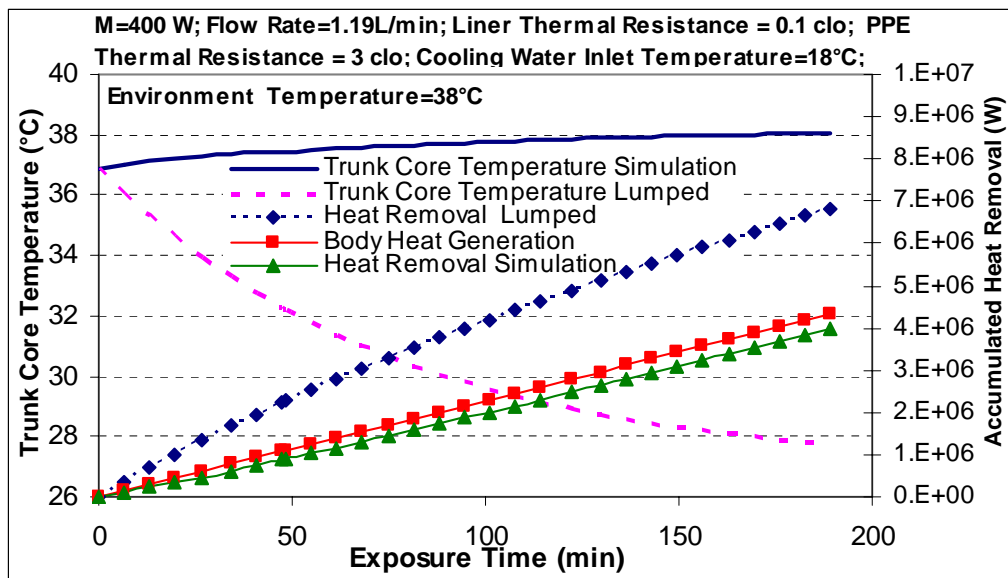
Figure 5.1 Comparisons of Trunk Core Temperature and Accumulated Heat Removal Predicted by Lumped Model and Thermal Model
