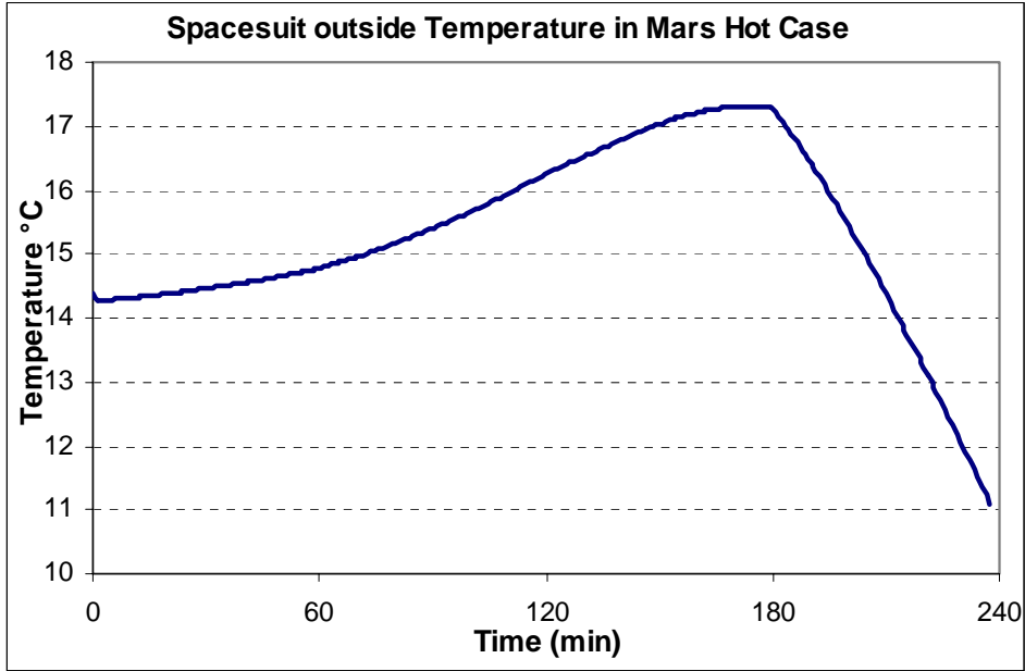
Figure 5.21 Outside Temperature of Spacesuit (Hot Case)
