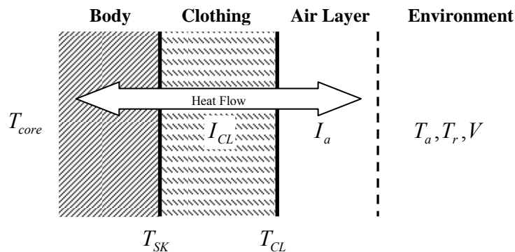
Figure 2.1 A Simple Model with a Layer of Clothing Insulation
