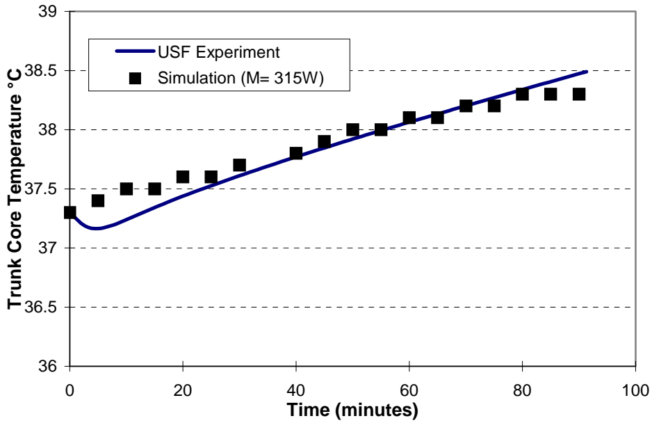
Figure 4.5 Comparison on Water Cooling Jacket between Simulation and USF Experiment—Subject A (M=315 W)
