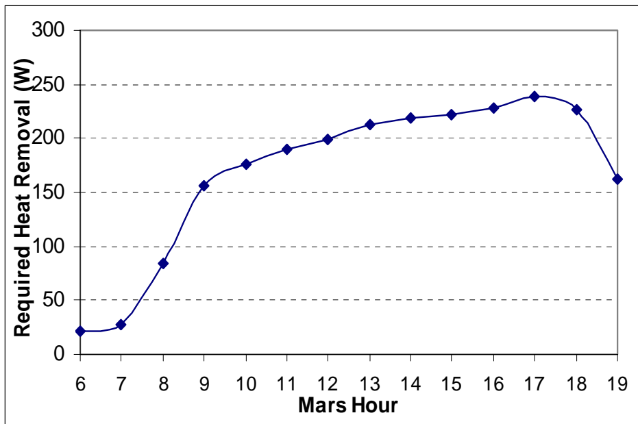
Figure 5.24 Required Heat Removal for Hot Case on Mars
