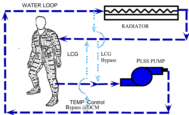
Figure 5.26 Simplified Flow Schematic Shuttle EMU with Radiator
