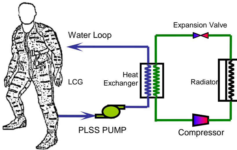
Figure 5.27 Simplified Flow Schematic Shuttle EMU with MVCC
