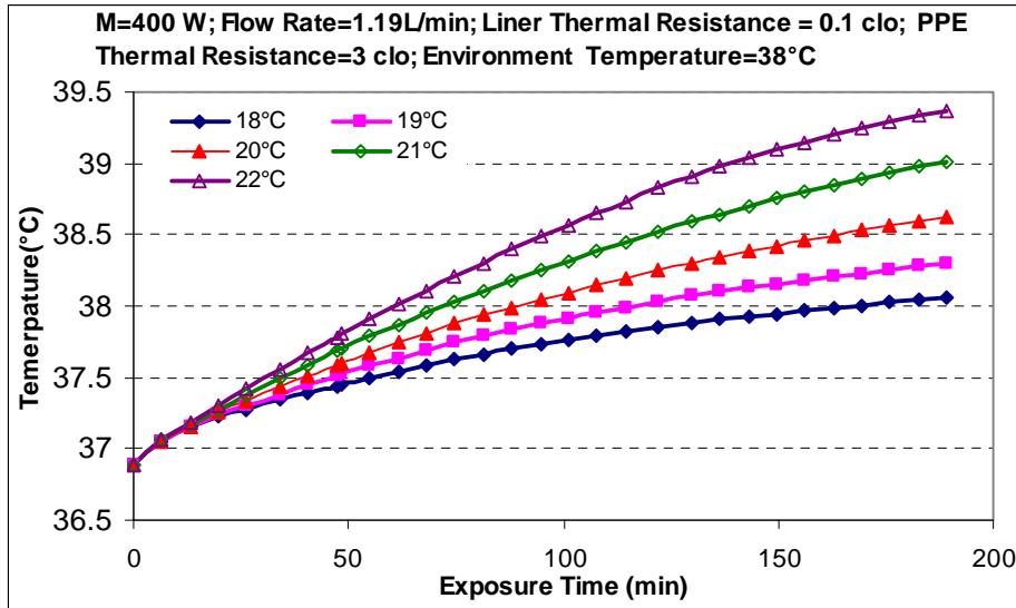
Figure 5.5 Trunk Core Temperature vs. Cooling Water Inlet Temperature
