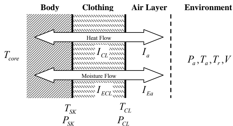
Figure 2.2 2-Parameter Model with a Layer of Clothing Insulation
