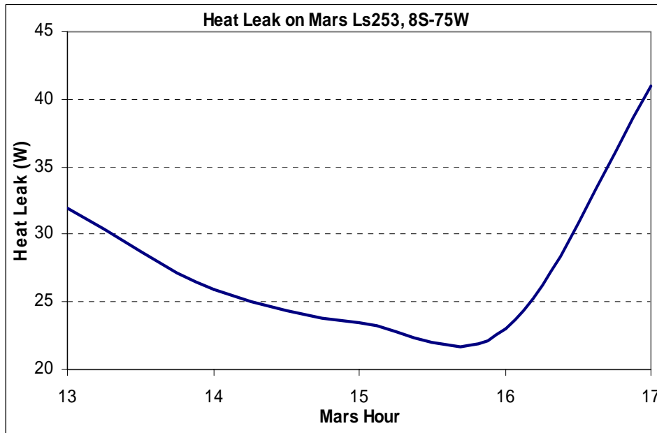
Figure 5.19 Heat Leak from Human Body to Environment (Hot Case)
