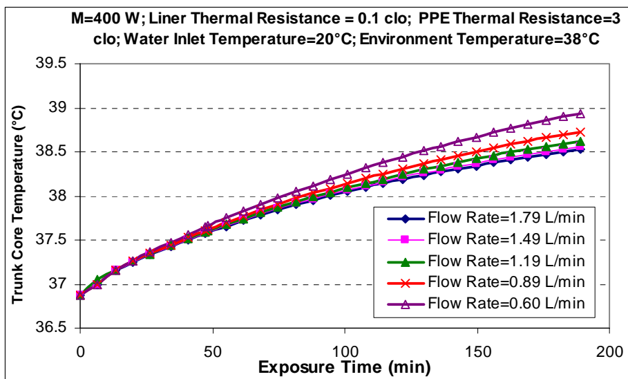
Figure 5.6 Trunk Core Temperature vs. Cooling Water Flow Rate
