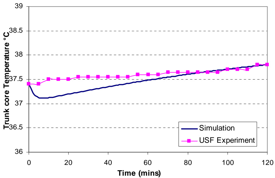
Figure 4.7 Comparison on Water Cooling Suit between Simulation and USF Experiment—Subject A (M=277 W)
