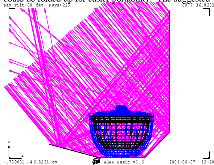
Figure 1. Ray trace of incident solar rays reflected from spherical mirror in red onto cooking pot in black, 40 degree solar altitude angle.
