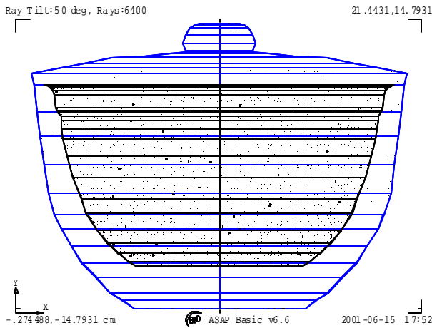
Figure 19. Spot diagram showing projections of ray intersections with cook pot onto the Y-X plane. Solar angle 50°.
