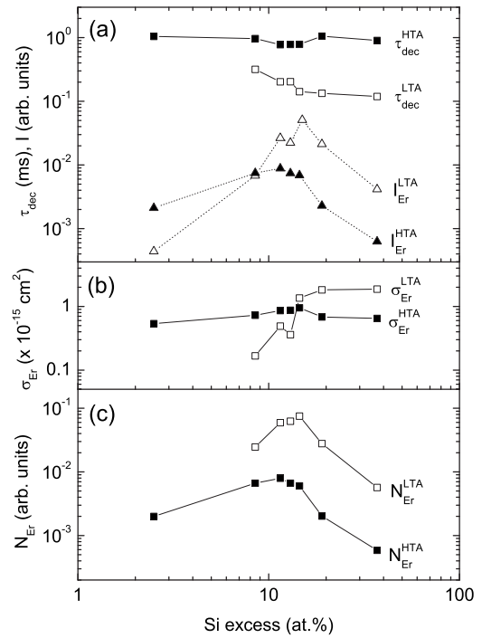
FIG. 2. (a) PL intensity of the \text{Er}^{3+} transition {}^4I_{13/2} \rightarrow {}^4I_{15/2} integrated in the region of 1350–1700 nm I and the \text{Er}^{3+} PL decay time at 1535 nm \tau_{\text{dec}} , (b) excitation cross section of the first excited state of \text{Er}^{3+} \sigma_{\text{Er}} , and (c) density of sensitized \text{Er}^{3+} ions N_{\text{Er}} of LTA and HTA samples as a function of Si excess concentration.
