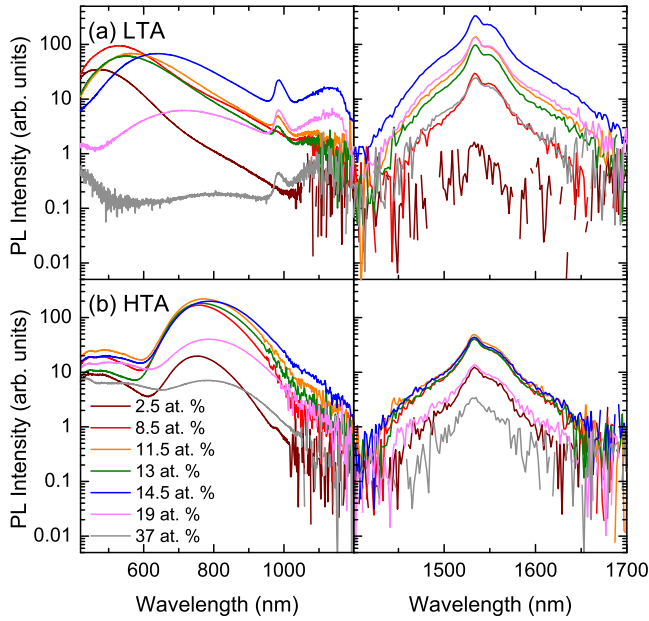
FIG. 1. (Color online) PL spectra of LTA (a) and HTA (b) samples with different silicon excess concentrations.
