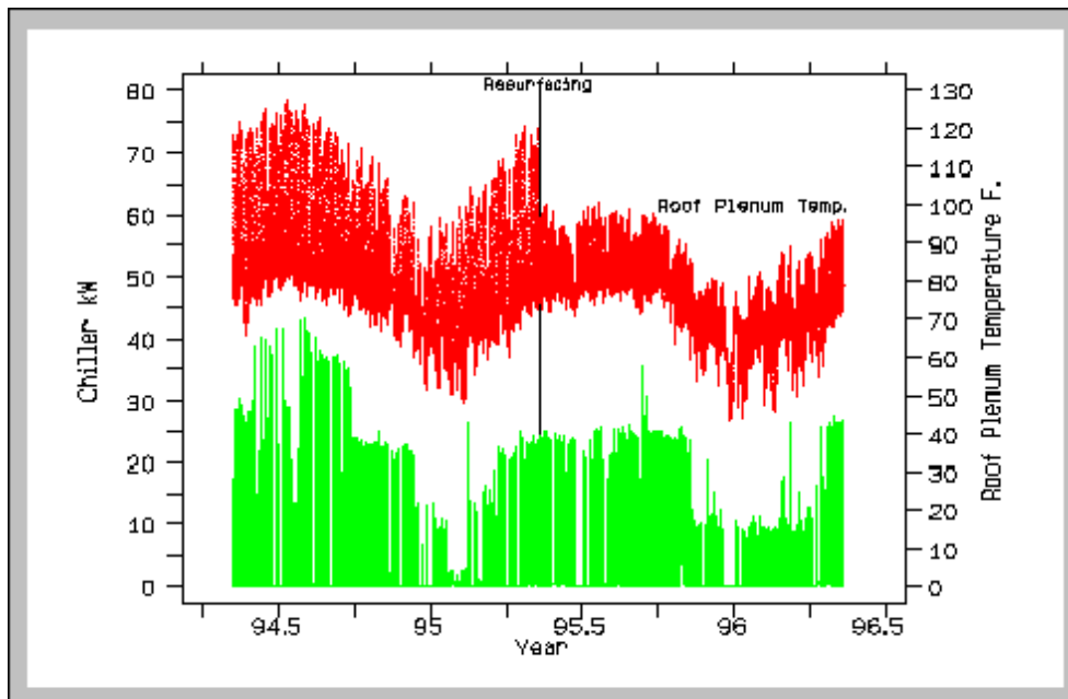
Figure 15. Data for two year period showing change in roof plenum thermal performance against 15-minute chiller electrical demand.
