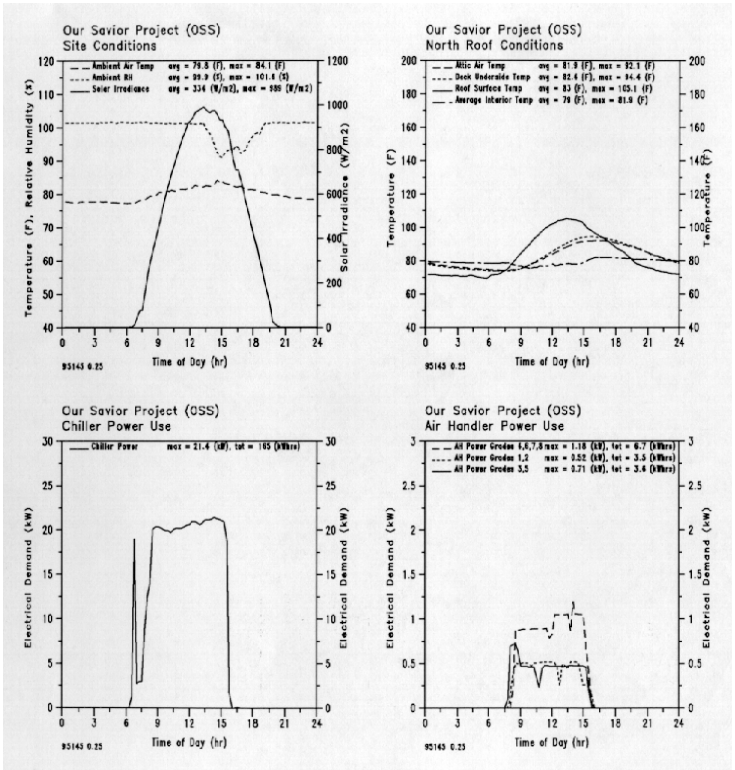
Figure 10. Measured thermal conditions and energy use at school after roof resurfacing -- May 25, 1995.
