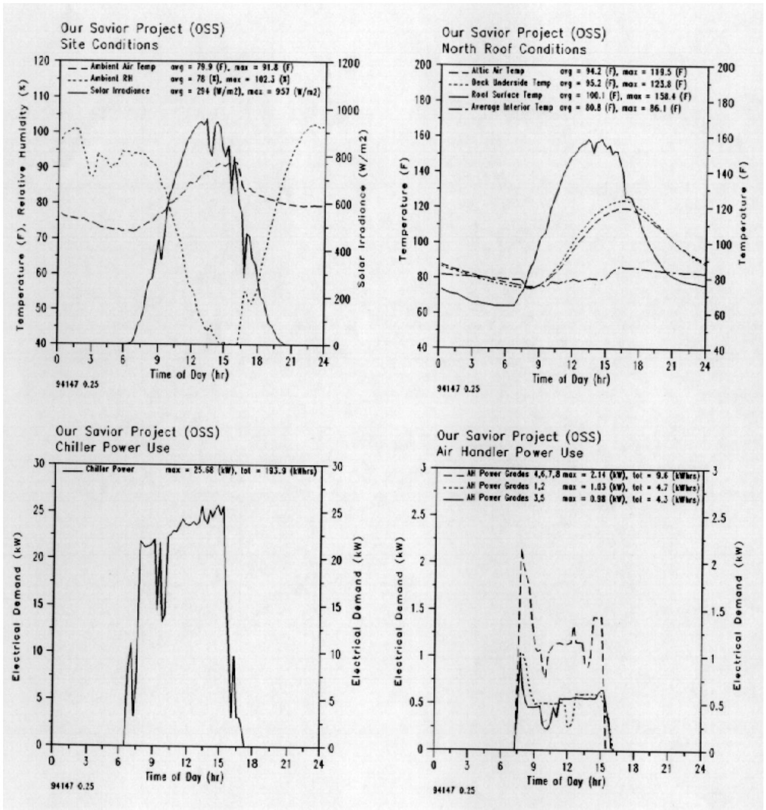
Figure 9. Measured thermal conditions and energy use at school prior to roof whitening-- May 27, 1994.
