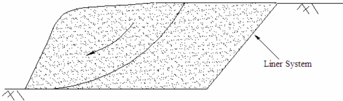
Figure 6: Failure within waste mass
