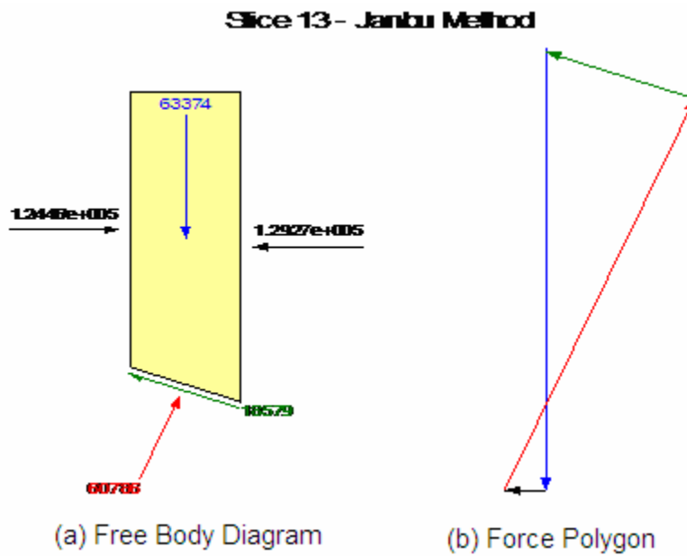
Figure 17: Summation of forces acting on a sample slice
