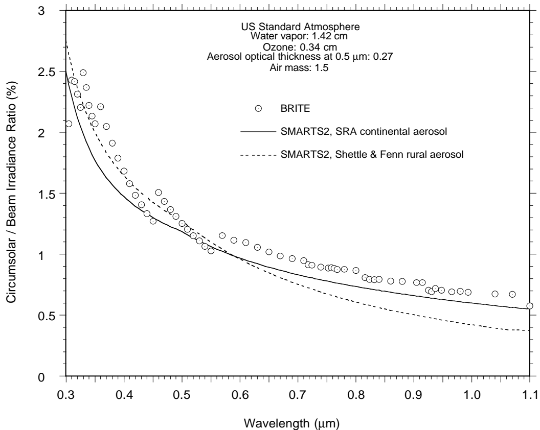
Fig. 8.7. Relative contribution of circumsolar radiation as predicted by SMARTS2 and BRITE for the conditions of the ASTM/ISO standards.
