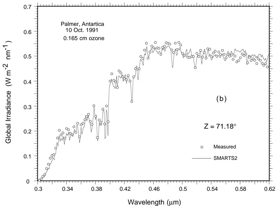
Fig. 8.12. Global irradiance predicted by SMARTS2 compared to actual UV measurements during a cloudless Spring day at Palmer, Antarctica (lat. 64.77^\circ S , long. 64.05^\circ W , alt. 13 m amsl). (a) UV-B data; (b) UV and visible data.
