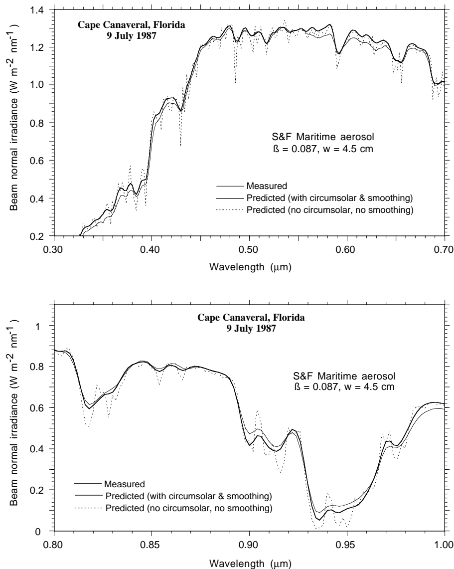
Fig. 8.15. Predicted vs measured beam normal irradiance at Cape Canaveral, Florida (lat. 28.42^{\circ}N , long. 80.61^{\circ}W , alt. 7 m amsl).
