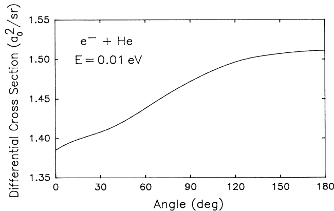
FIG. 1. Differential cross sections at 0.01 eV.
