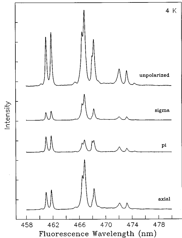
FIG. 8. Polarized emission spectra (transverse and axial) from the ^1D_2 to the ^3F_4 multiplet manifold at 4 K.
