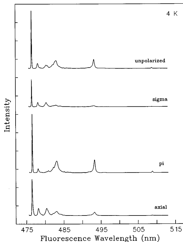
FIG. 5. Polarized emission spectra (transverse and axial) from the ^1G_4 to the ^3H_6 multiplet manifold at 4 K.
