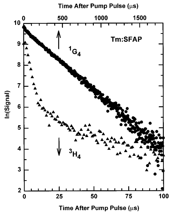
FIG. 9. Room temperature fluorescence decay waveforms for Tm:SFAP ^1G_4 and ^3H_4 fluorescence following pulsed excitation. The upper time scale applies to the ^1G_4 decay, the lower scale to the ^3H_4 decay.
