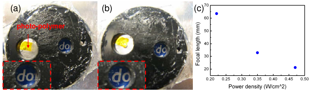
Fig. 4. (a) Liquid lens at non-focusing state, (b) Liquid lens at a focusing state, and (c) Measured focal length of the lens at different power densities.
