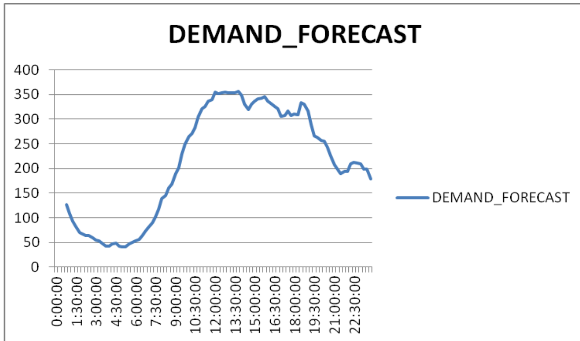
Figure19. EWMA Forecast
