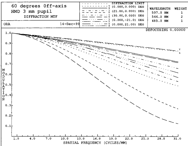
Fig. 2 Plots of the polychromatic MTF for a 3-mm pupil size and various points in the field of view. Plots are shown up to 31.25 lp/mm, corresponding to a pixel size of 16 \mu\text{m} ; 20 lp/mm corresponds to 25- \mu\text{m} rms spot size, the desired performance.
