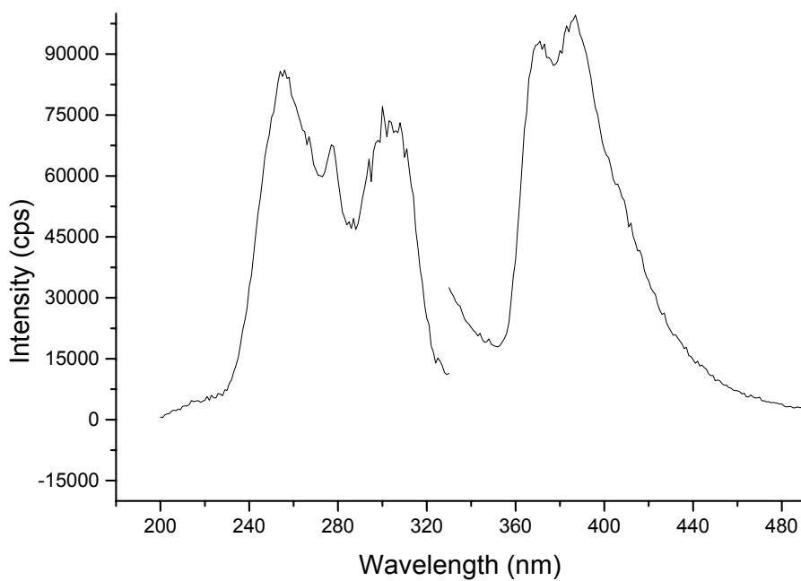
Figure 3.4A. Room temperature excitation and fluorescence spectra of 100 ng/mL 9-OHpe in methanol/water (0.05% v/v)
