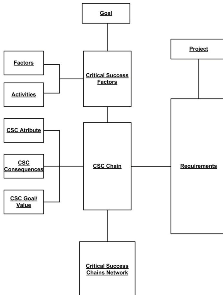
Figure 4.10: CURE meta-model
