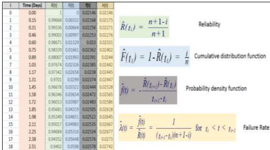
Figure 5-14: F(t) , R(t) , f(t) , and \lambda(t) for failure data
