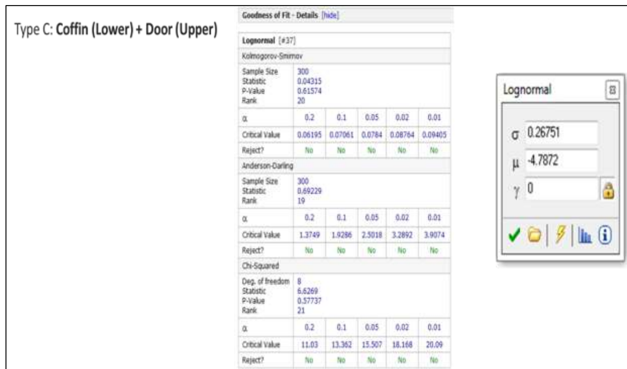
Figure 5-17: Probability destitution for refrigerator Type C
