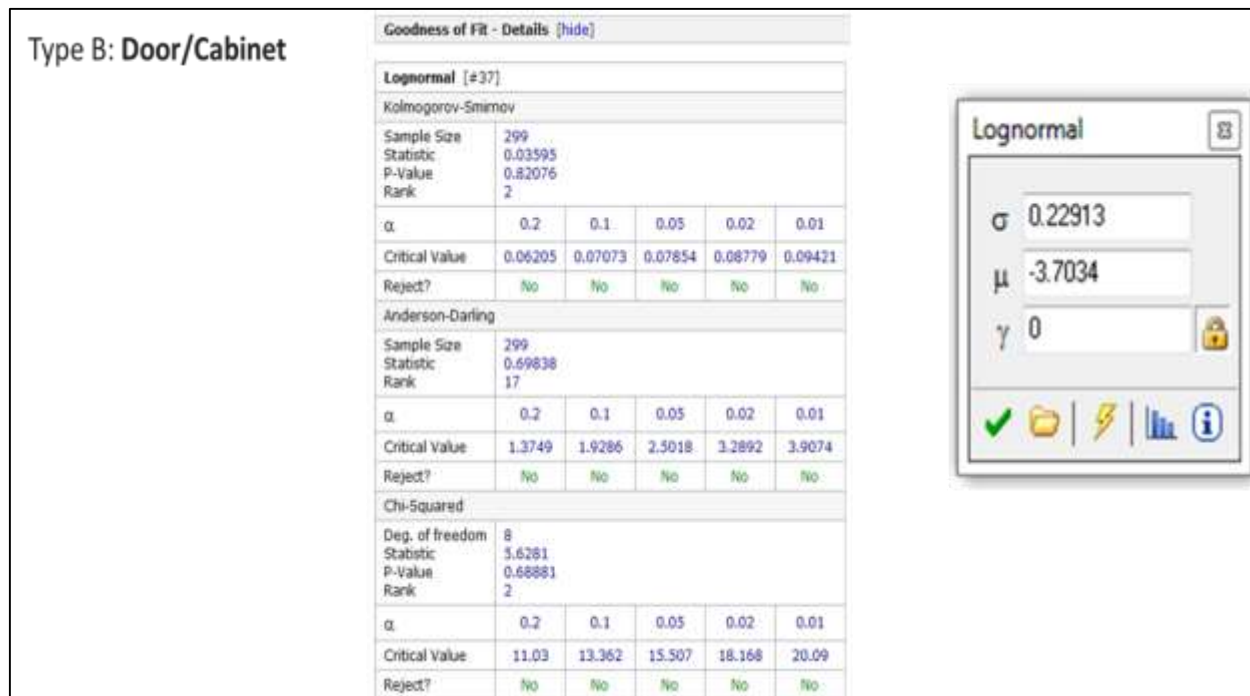
Figure 5-16: Probability destitution for refrigerator Type B
