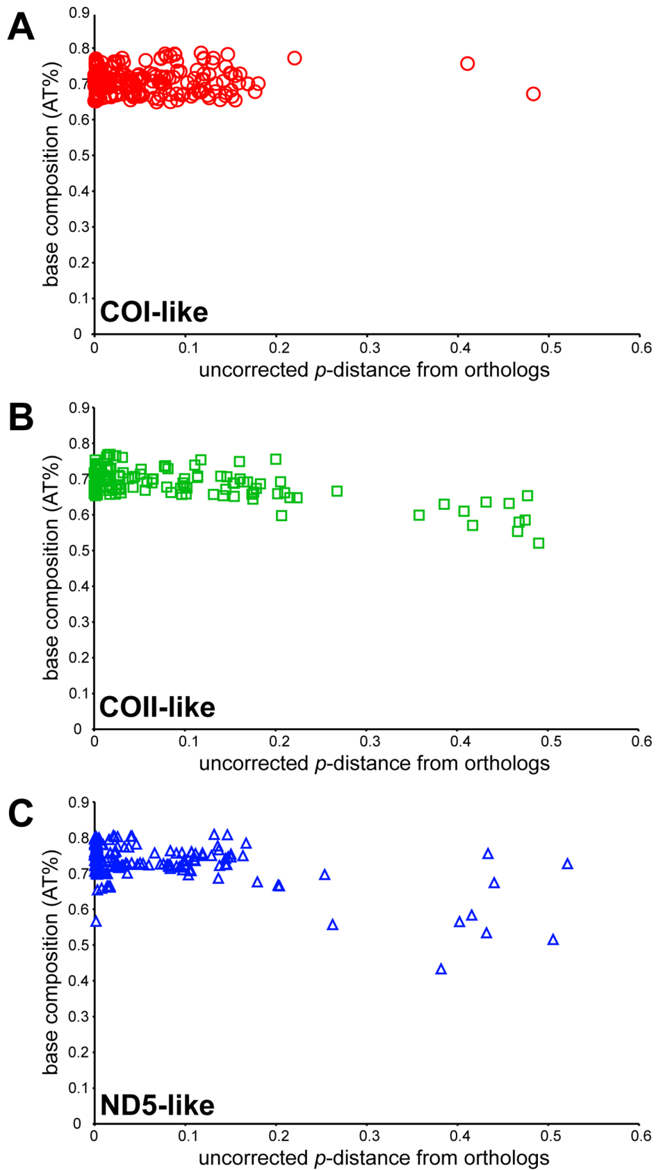
Figure 2. Characteristics of numts as measured by base composition and uncorrected p -distance from orthologs. A: COI-like numts; B: COII-like numts; C: ND5-like numts. doi:10.1371/journal.pone.0110508.g002
