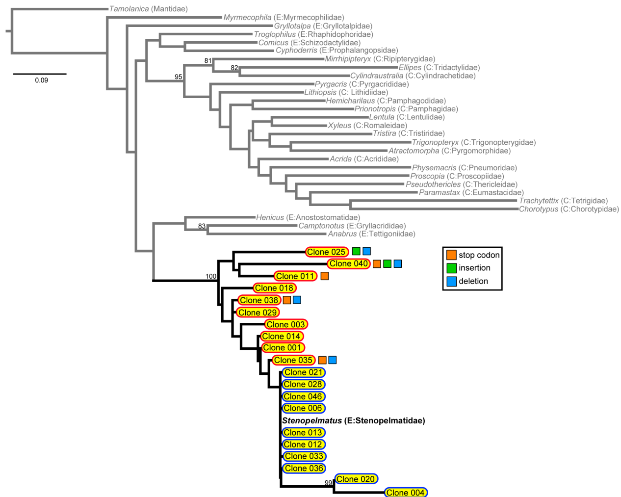
Figure 3. Co-analysis of numts and mtDNA using COI-like numts of Stenopelmatus fuscus (Ensifera: Stenopelmatidae). Grey terminals represent orthologous COI across Orthoptera. The maximum likelihood analysis recovered a monophyletic group consisting of COI-like numts and the ortholog from S. fuscus . Paleonumts are denoted by yellow with red outline, and neonumts are denoted by yellow with blue outline. Those numts with premature stop codons, insertions, and deletions, are indicated by orange, green, and blue squares, respectively. Numbers on nodes indicate bootstrap support values.
