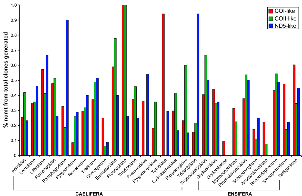
Figure 1. Numts of three mitochondrial genes (COI, COII, ND5) are extremely abundant across the phylogenetic diversity within Orthoptera. The y-axis shows the proportion of numts from the total number of clones generated based on PCR using conserved primers. If nearing 1, most clones generated are numts. If nearing 0, most clones generated are orthologous mtDNA. doi:10.1371/journal.pone.0110508.g001
