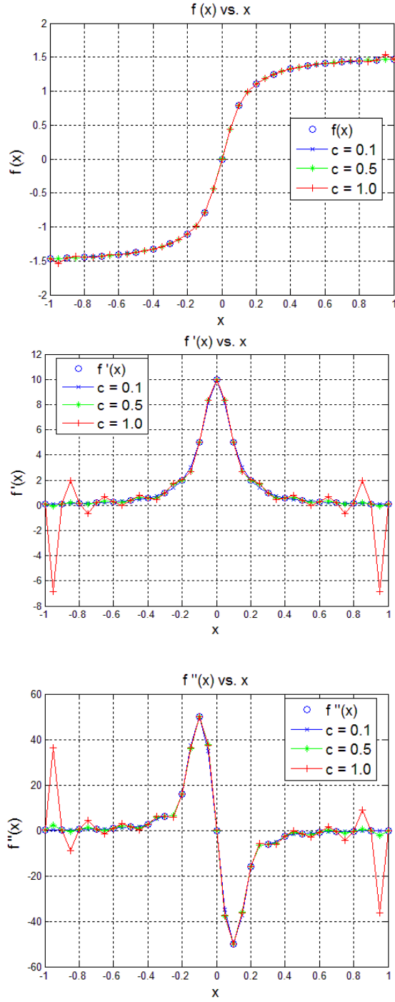
Figure 11: Test function f(x) = A \tan^{-1}[\omega(x - x_0)] A = 1 \omega = 10
